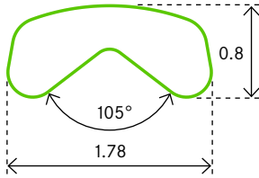
PROFILE 0783 Stainless Steel
