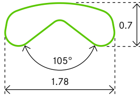
PROFILE 0784 Stainless Steel
