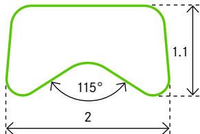
PROFILE 0184 Monel
