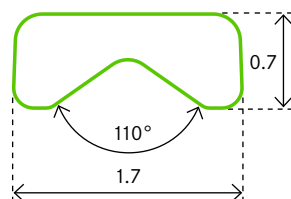
PROFILE 0770 Stainless Steel
