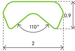
PROFILE 0553 Monel/Stainless Steel
