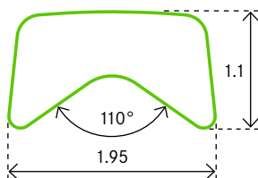
PROFILE 0369 Monel/Stainless Steel
