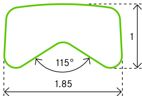
PROFILE 0150 Monel
