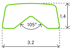
PROFILE 0309 Monel
