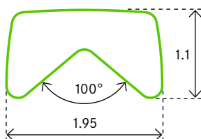
PROFILE 0314 Monel/Stainless Steel
