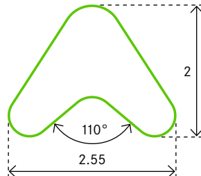
PROFILE 0315 Monel/Titan
