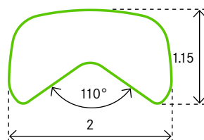
PROFILE 0528 Monel
