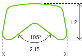
PROFILE 0361 Monel
