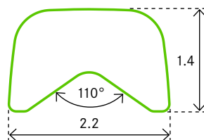
PROFILE 0389 Stainless Steel
