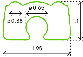
PROFILE 0539/LS41 Monel
