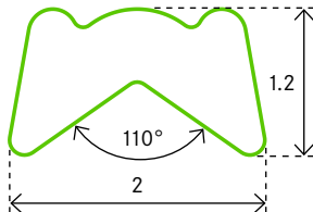
PROFILE 0208 Monel
