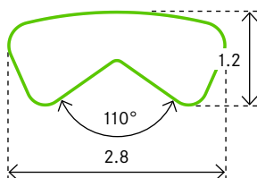
PROFILE 0453 Monel
