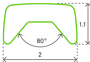
PROFILE 0988 Monel
