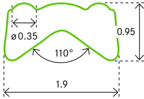
PROFILE 0538/S41 Monel/Stainless Steel
