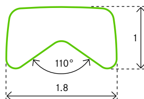
PROFILE 0315 Monel/Titan
