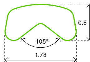
PROFILE 0782 Monel/Stainless Steel
