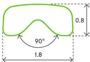
PROFILE 0447 Monel/Stainless Steel/Titanium
