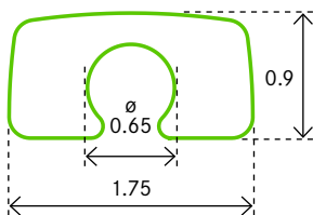
PROFILE 0555 L Monel/Stainless Steel/Titanium
