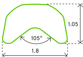
PROFILE 0463 Monel
