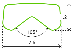
PROFILE 0768 Monel
