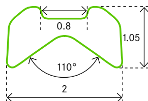
PROFILE 0686 Monel
