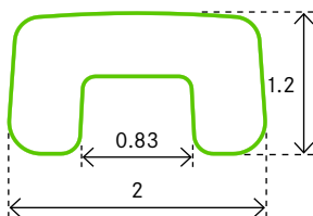
PROFILE 0848 U Monel/Stainless Steel
