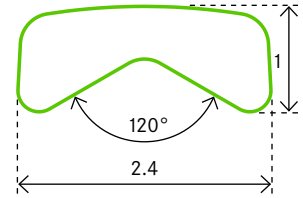
PROFILE 0832 Monel
