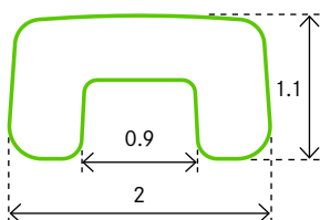
PROFILE 0288 U Monel/Stainless Steel
