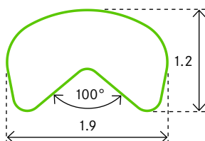
PROFILE 0518 Monel
