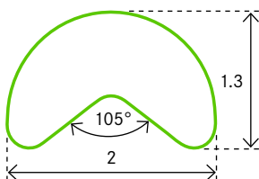
PROFILE 0597 Monel
