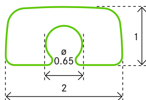
PROFILE 0681 L Monel/Stainless Steel/Titanium
