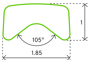
PROFILE 0363 Monel
