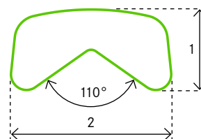
PROFILE 0702 Monel
