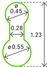
PROFILE N 102 Nylon
