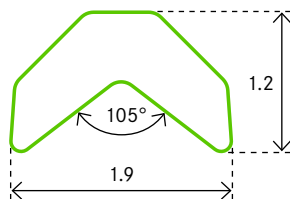
PROFILE 0556 Monel
