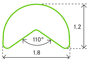
PROFILE 0469 Monel
