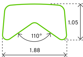
PROFILE 0678 Monel/Stainless Steel
