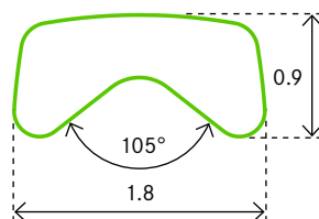
PROFILE 0455 Monel/Stainless Steel
