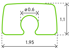
PROFILE 0435 L Monel/Stainless Steel/Titanium
