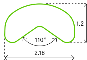
PROFILE 0677 Monel
