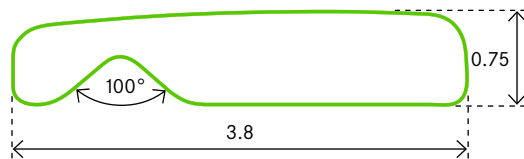
PROFILE 8020 Monel
