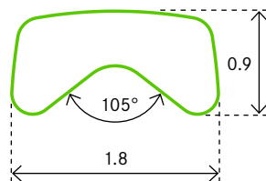
PROFILE 0572 Monel
