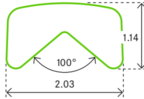
PROFILE 0825 Monel
